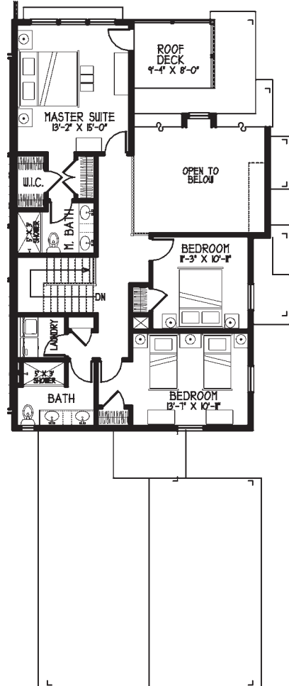
SECOND FLOOR = 934 SQ. FEET
