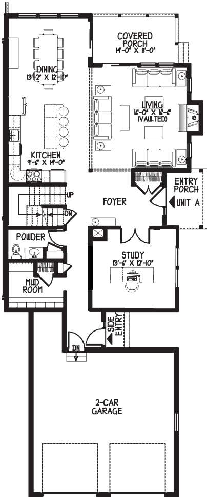
FIRST FLOOR = 1308 SQ. FEET
